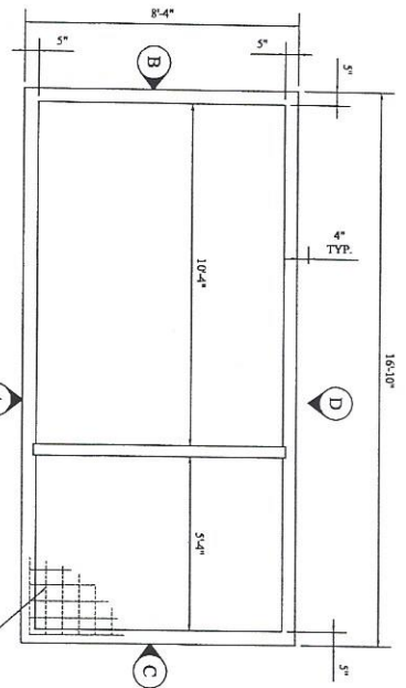
PLAN - BOTTOM SLAB
