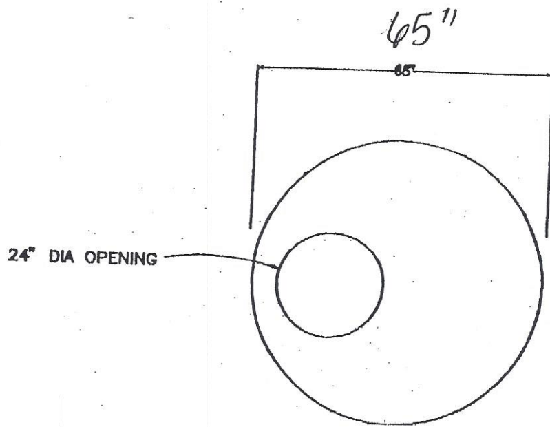
COVER PLAN
