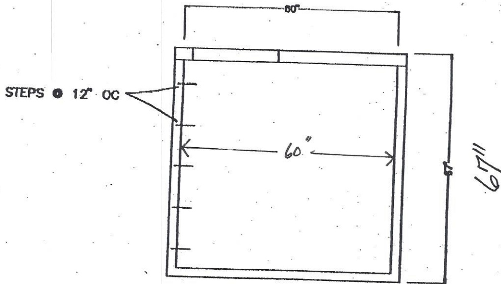
INTERIOR SECTION
